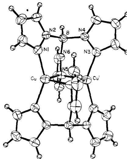
Figure 1. The molecular geometry of the centrosymmetric dimer [Cu(HBpz 3 ) 2 ].
